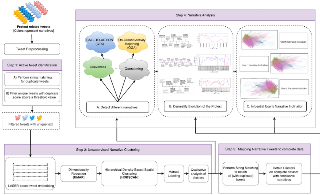
Figure 4.2: Proposed framework to demystify protest composition. The framework is divided into 4 parts. First, we identify the active tweets for the protest. Second, we utilize a clustering-based method for unsupervised narrative detection. Next, we map the narrative tweets to complete data. Finally, we perform the narrative analysis on the complete data.
