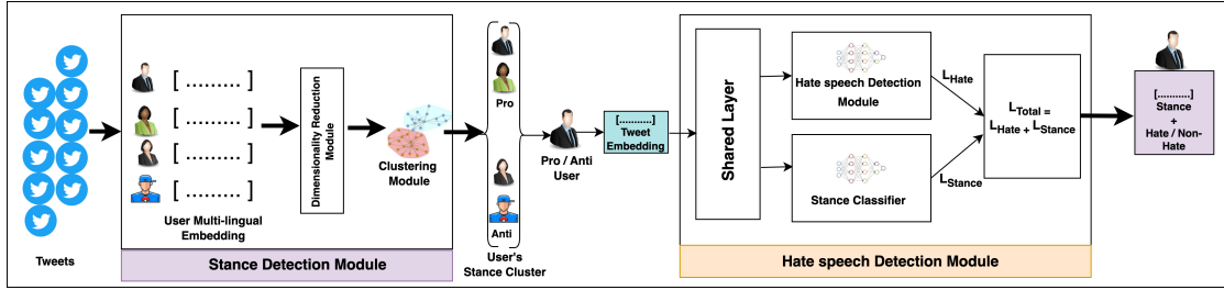
Figure 6.2: Figure showing our proposed framework to detect user-level stance followed by tweet-level hate speech detection for stance-aware users.
