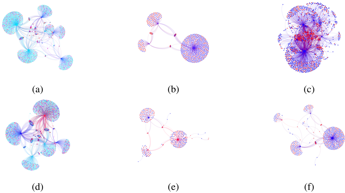
Figure 6.5: Figure showing Retweet network of users' interaction with different hate intensities for CP and P users. The size of the nodes corresponds to retweet frequency. Figure a-c presents the CP retweet network. Figure d-f presents the P retweet network. Color scheme: Dark blue: old low-intensity users, Light-blue: new low-intensity users, Red: old mid and high hate-intensity users, and Pink: new mid and high-intensity users. We find that the number of hateful users increased towards the most hateful day reported in tweets.
