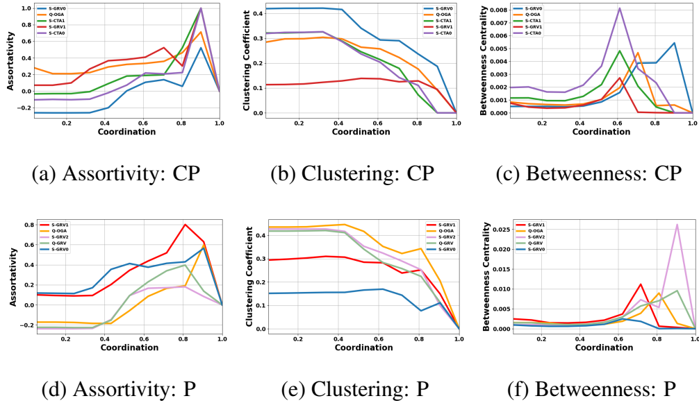
Figure 7.3: Figure showing the relationship between computed network measures for each coordinated community as a function of the extent of coordination.
