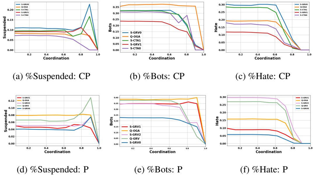
Figure 7.4: Figure showing the relationship between the percent suspended users, percent bots, and mean hate for each coordinated community as a function of the extent of coordination for the opposing stances.
