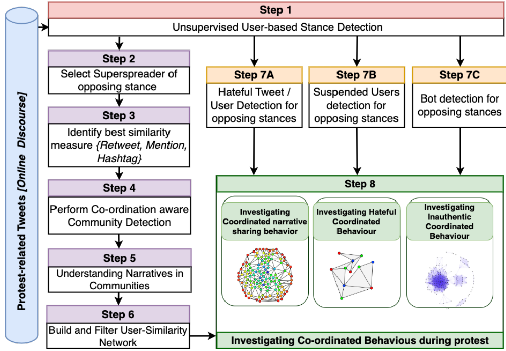
Figure 7.1: Overview of our approach based on combining the analysis of hateful user detection and various inauthentic activities with coordination for examining coordinated harmful behavior.
