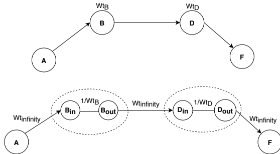
Fig. 4: Vertex Splitting
