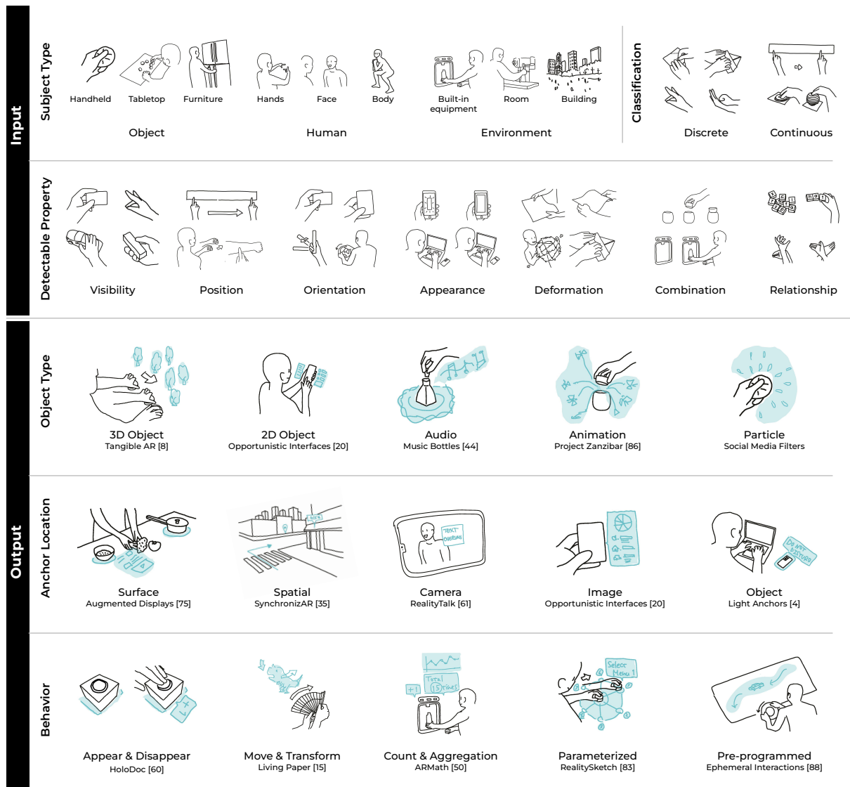
Figure 6.2: Design space of supported modalities of input and output for tangible AR prototypes.
