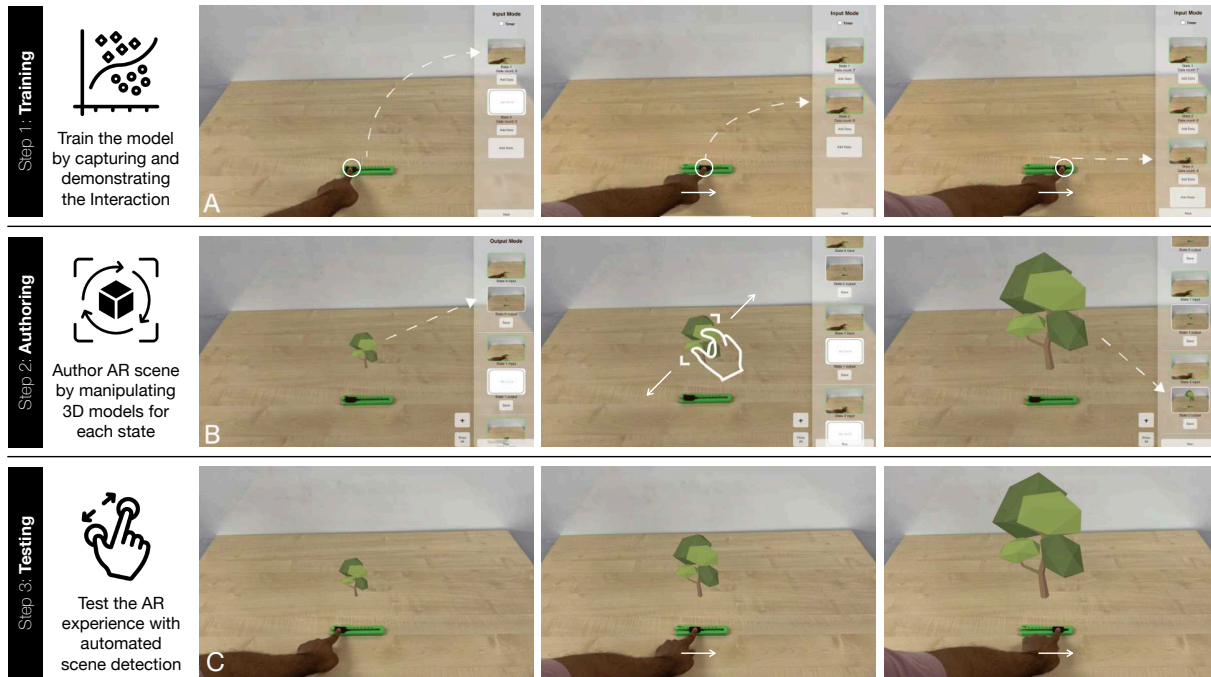
Figure 4.1: Authoring Workflow of Teachable Reality: Using a paper cutter as a slider to control the scale of a virtual tree: A) User captures three states of the everyday object while demonstrating the tangible interaction. B) User saves the output of the virtual world corresponding to each input state. On importing the virtual asset, the user manipulates the virtual asset according to the desired output and saves it to every corresponding input state. C) User tests the created prototype, which animates between all the outputs that were saved.
